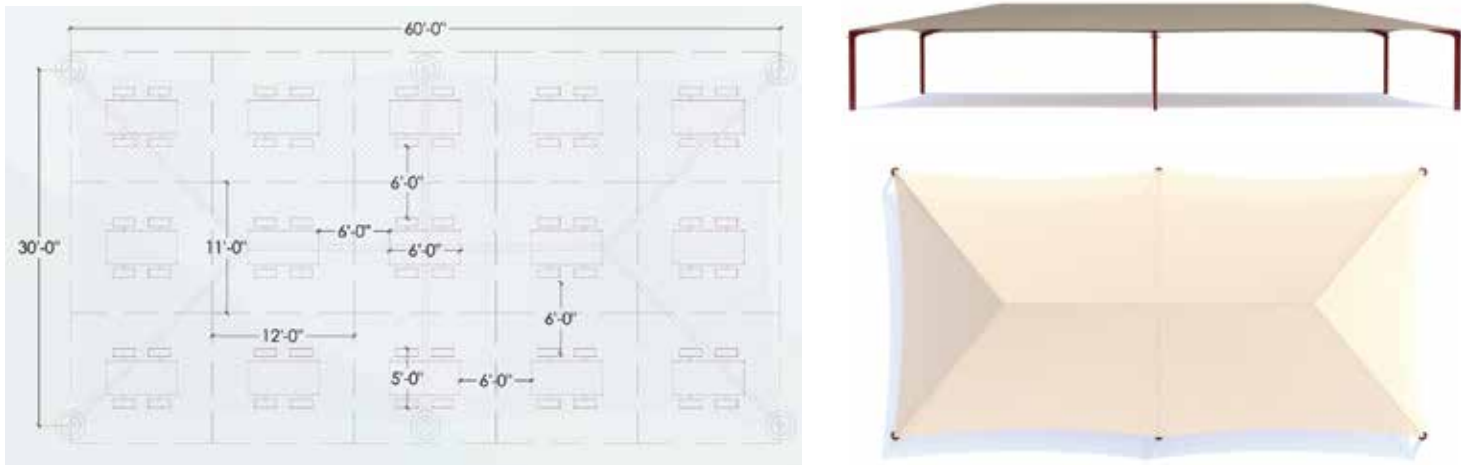
30' x 60' 6 Post Hip with Single Canopy Sits up to 60 students
